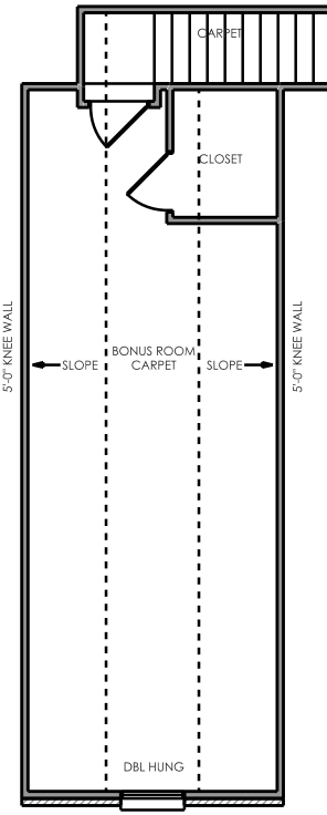
REC ROOM PLAN
