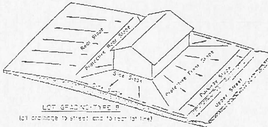
EXAMPLE: BLOCK GRADING TYPE 2 Single Cross Slope
