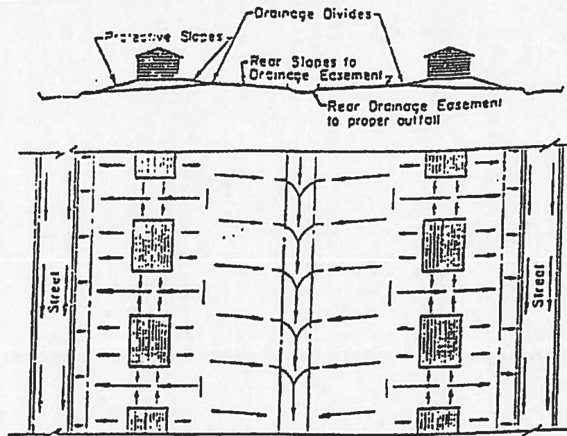
LOT GRADING - TYPE B
