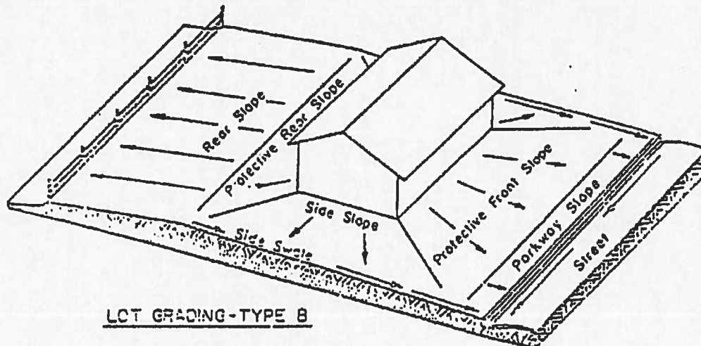
LOT GRADING - TYPE B
